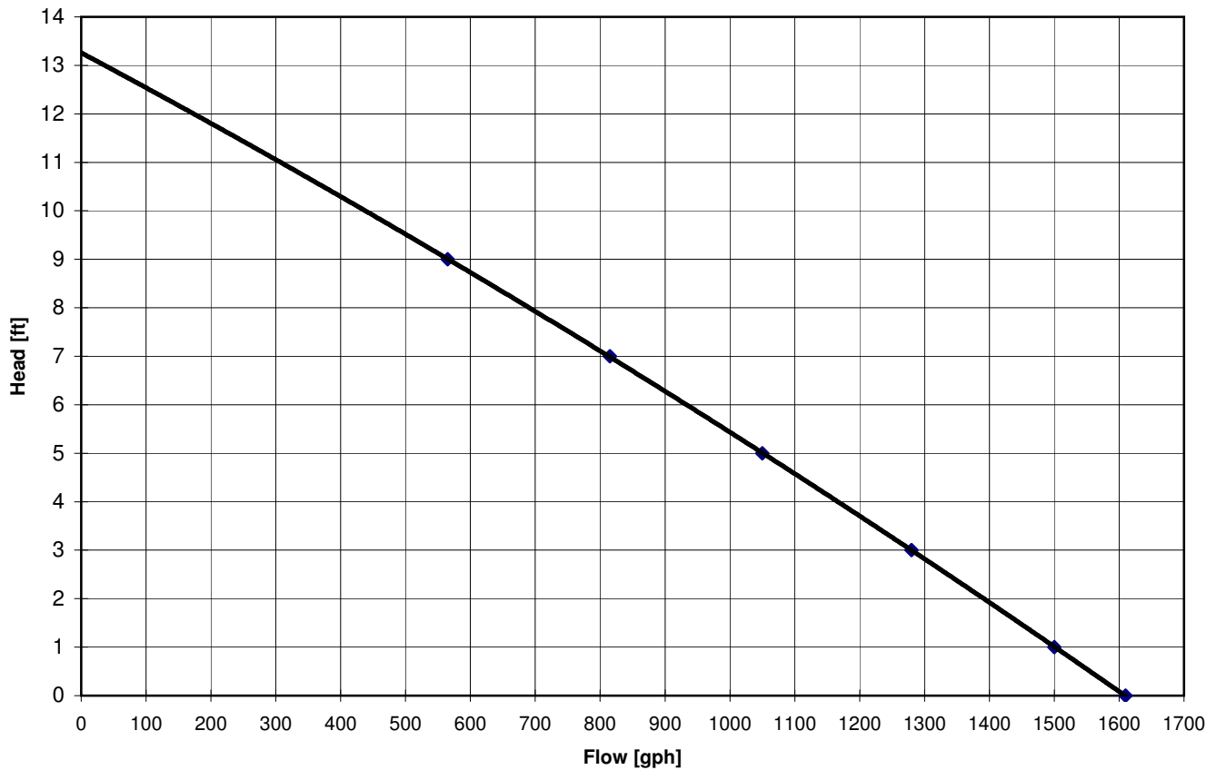
P1500 Pump Curve Magnetic Driven Pump
